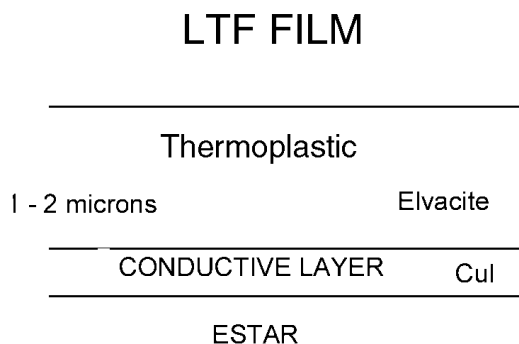
Figure 2. Cross section of recording substrate
